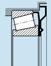
AK -A double externally sealing NILOS-Ring for a single-row 313 11 tapered roller bearing would be designated type 313 11 AK.
